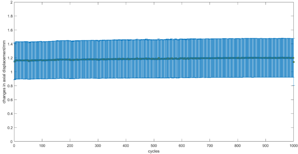
Figure S1: Mean and standard deviation of changes in axial displacement ( d ) during cyclic loading [30 1200 N] of all specimens implanted with COPAL knee spacers.
