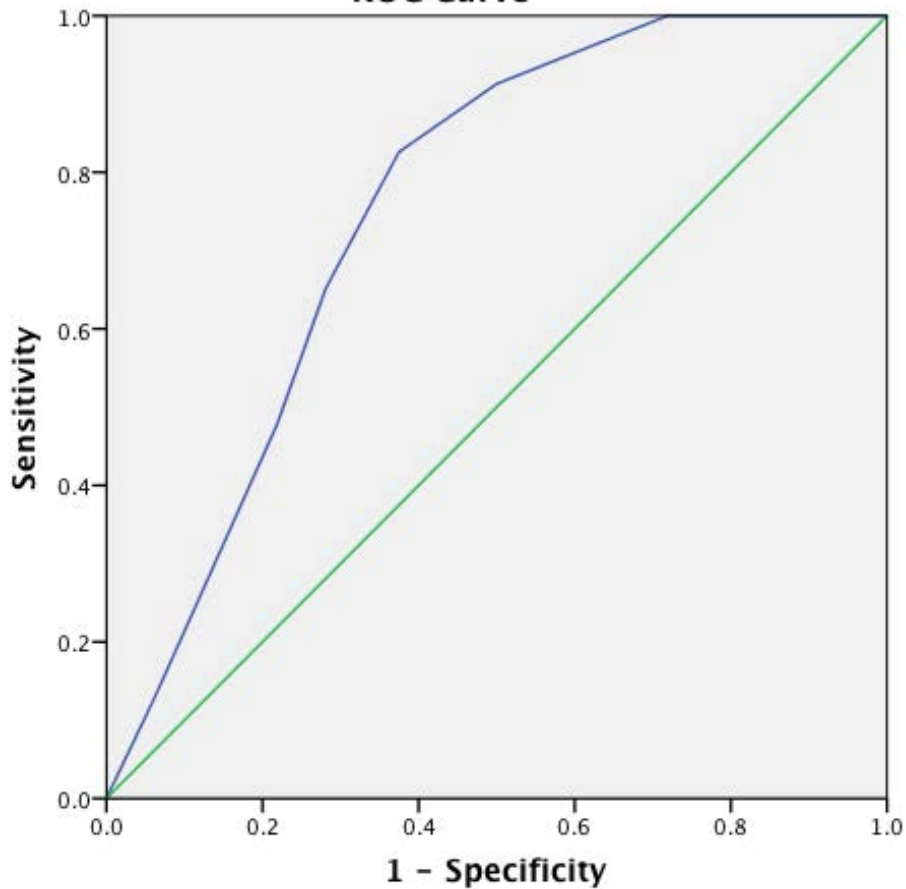
ROC Curve
