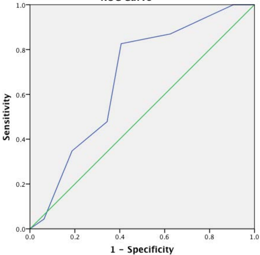
ROC Curve
