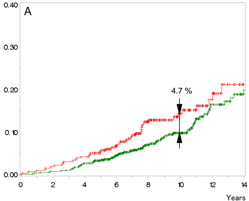
Cumulative incidence
