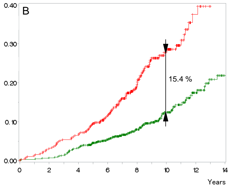
Cumulative incidence
