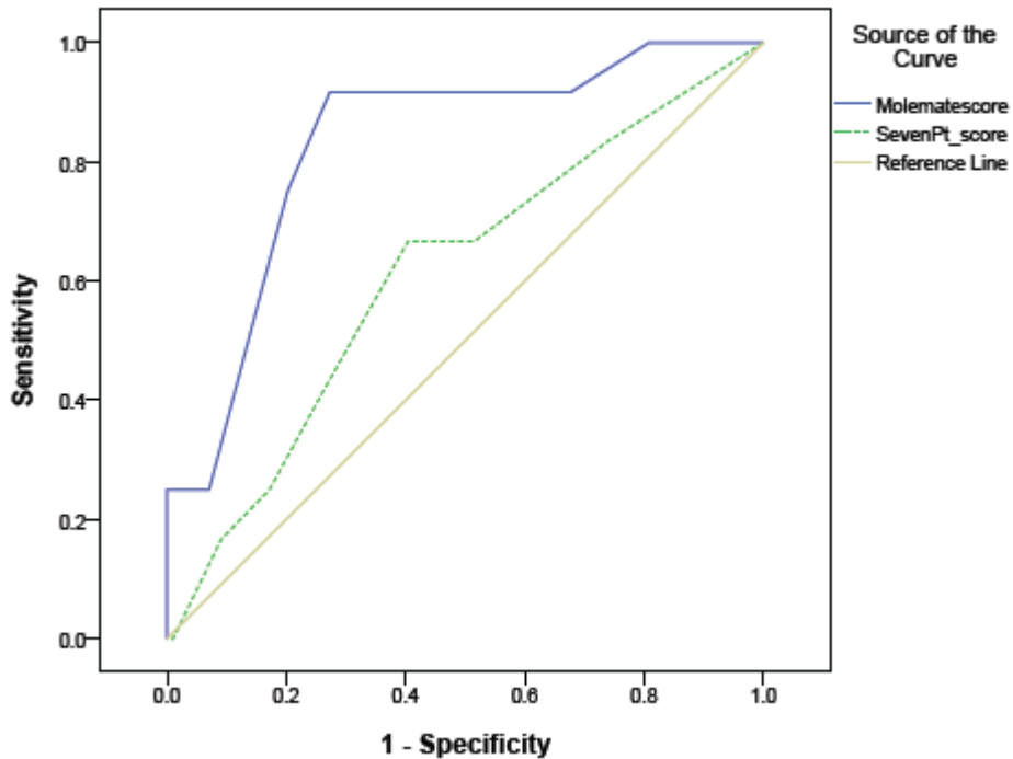
ROC Curve
