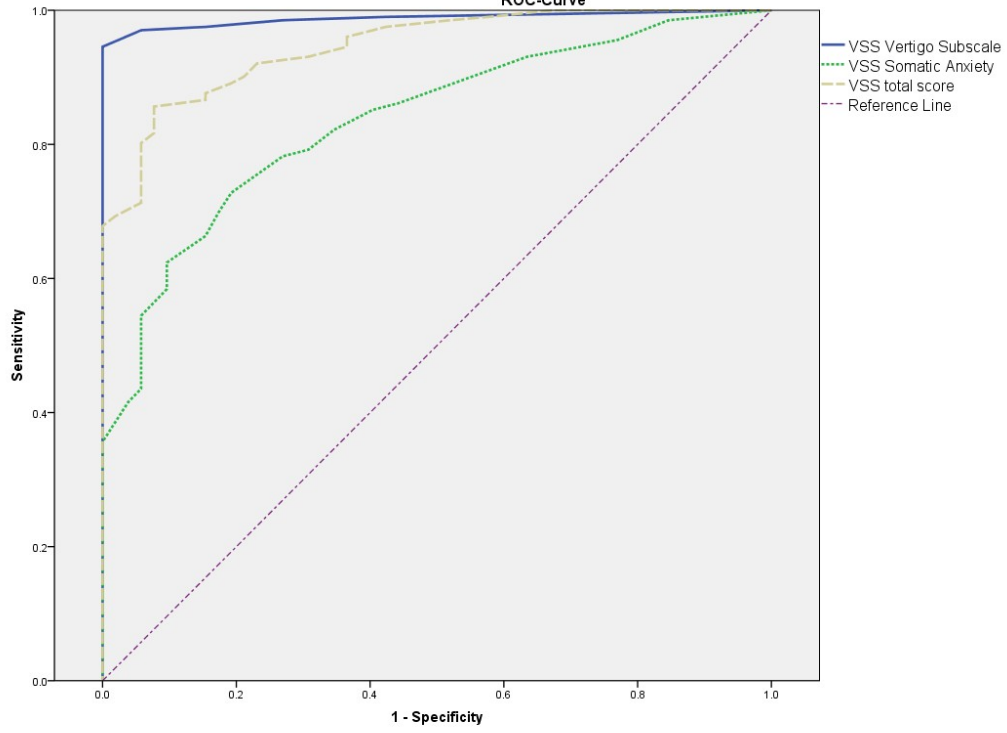
ROC-Curve
