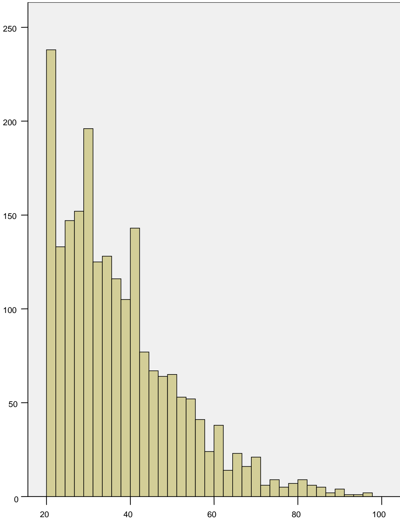
DFS scores
