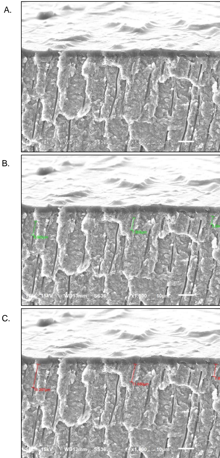
Figure S1 (A–C) Scanning electron micrographs of longitudinal views of intact dentin with fluoride iontophoresis and self-etch adhesive treatment (original magnification X1000), showing bundle precipitates with the size of 5-10 μm in dentinal tubules at the depth of 8-16 μm.
