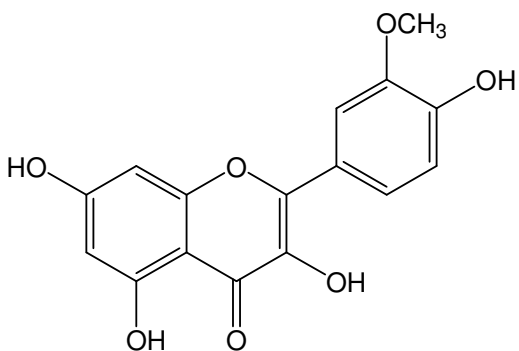
Compound C Isorhamnetin
