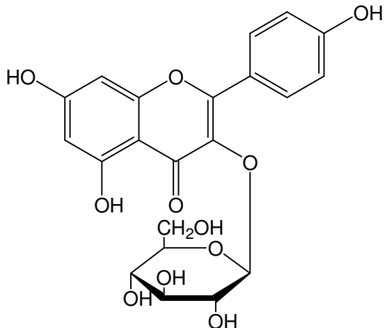
Compound B Kaempferol-3-Glucoside
