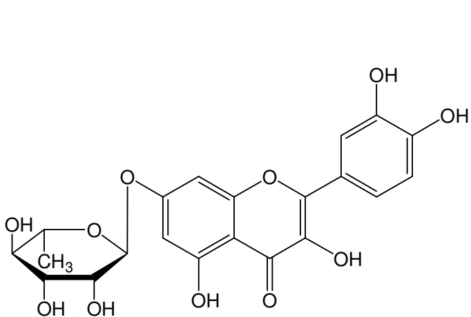
Compound A Quercetin-7-Rhamnoside
