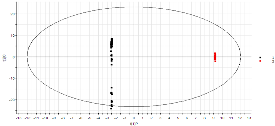
Scores Comp[1] vs. Comp[2] colored by Sample Group (original)
