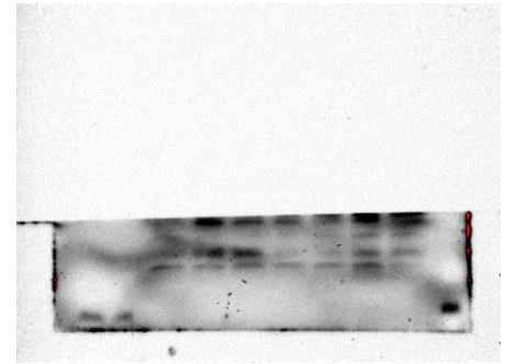
Cleaved caspase-3
