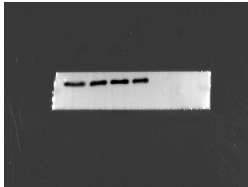
Lamin B1-③
