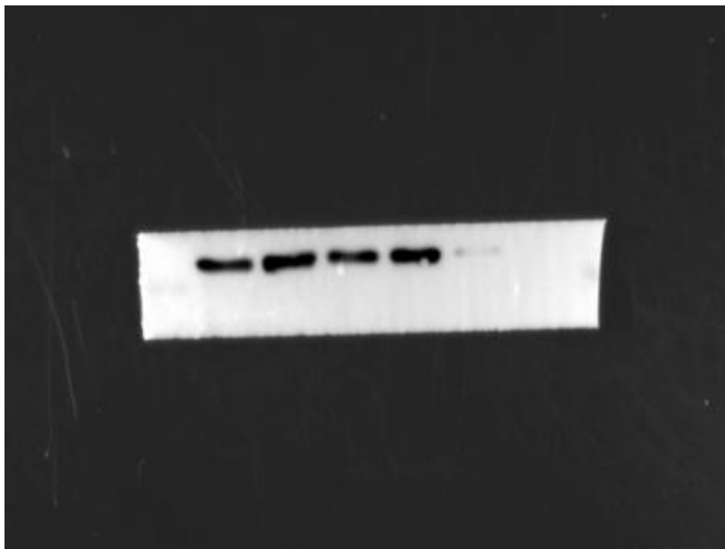
Lamin B1-②
