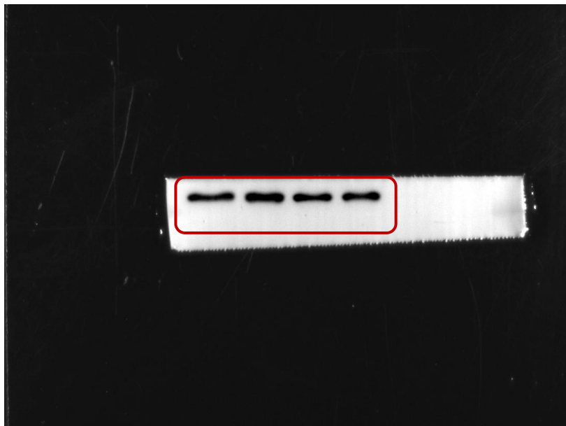
Lamin B1-①
