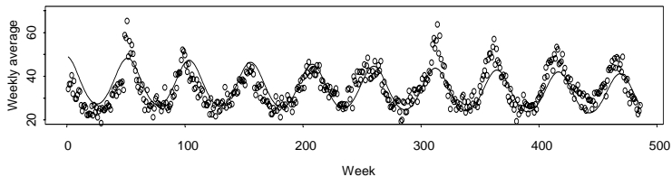
Simulated Data from Hierarchical Model
