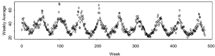
Simulated Data from Nonhierarchical Model
