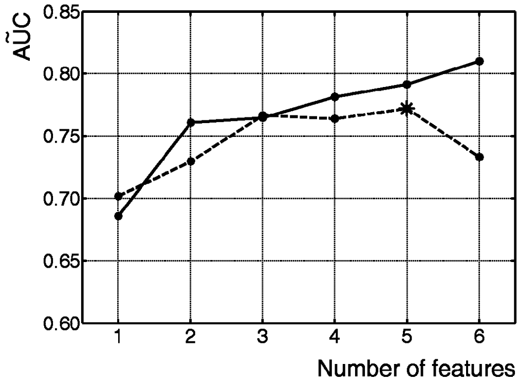
kNN model
