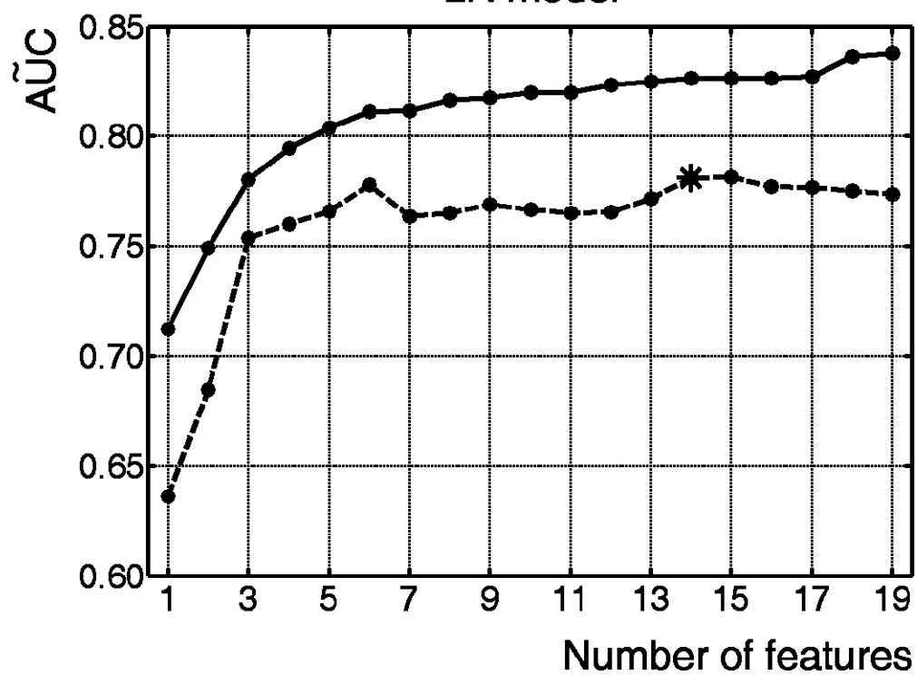
LR model
