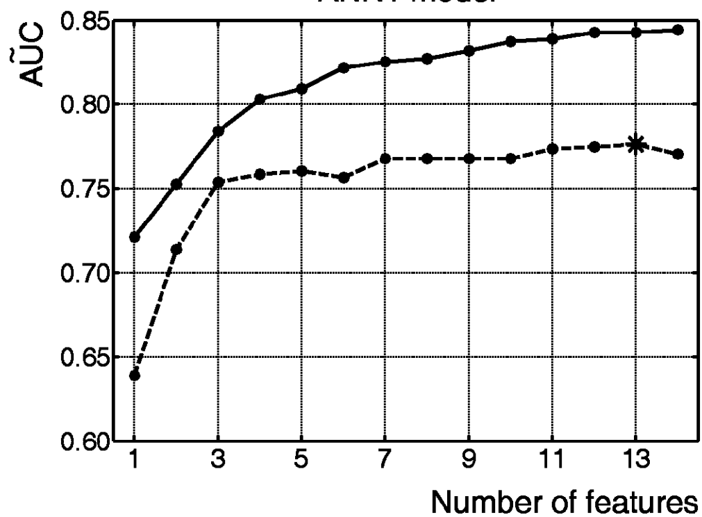
ANN1 model
