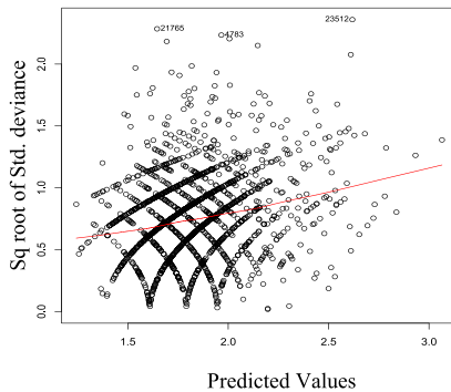
Scale-Location
