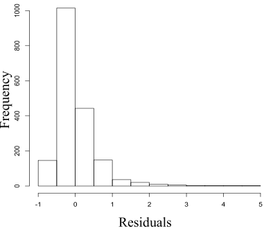
Histogram of Residuals
