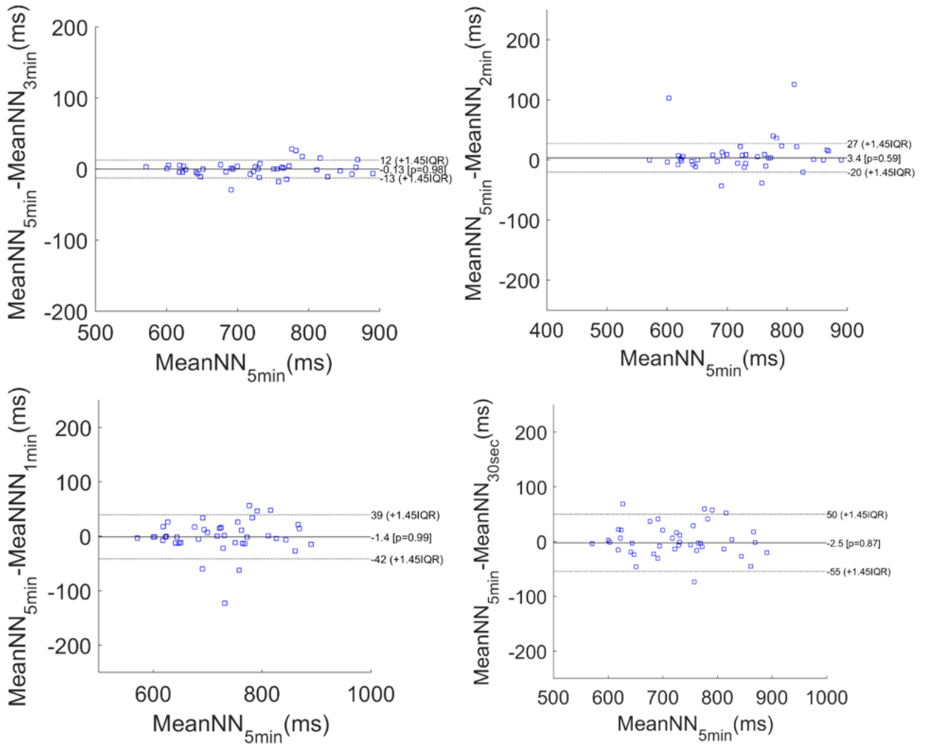
Fig. S1 Bland-Altman Plot of MeanNN during Rest. IQR: Interquartile range.
