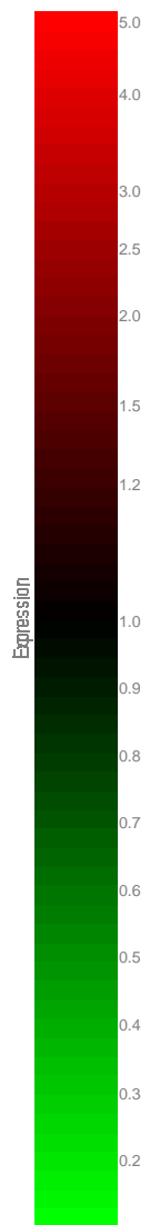
Cluster 4: 677 genes
