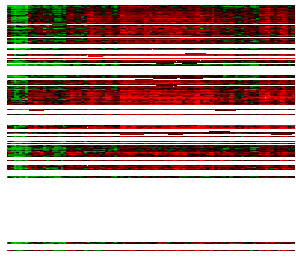
Cluster 1: 754 genes
