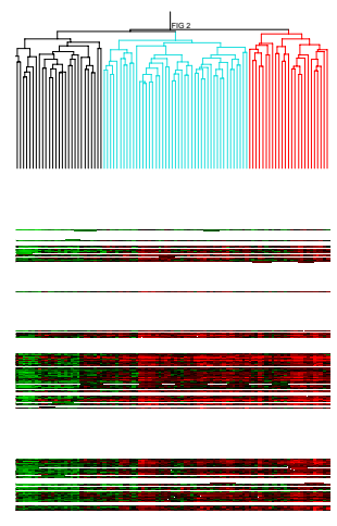
Cluster 5: 671 genes
