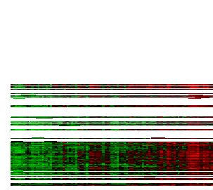
Cluster 4: 677 genes
