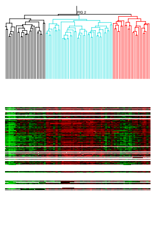
Cluster 9: 1054 genes
