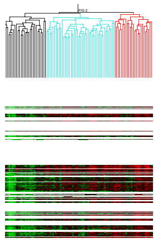
Cluster 8: 661 genes
