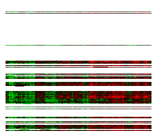
Cluster 2: 590 genes
