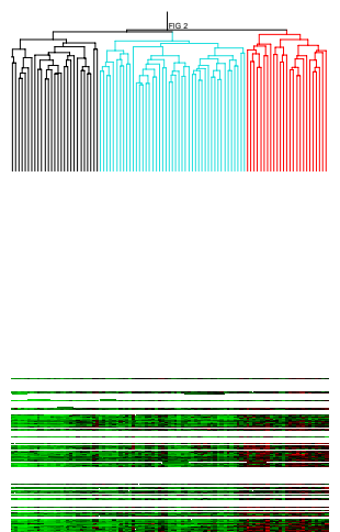
Cluster 7: 465 genes
