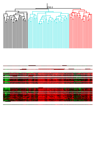
Cluster 6: 601 genes
