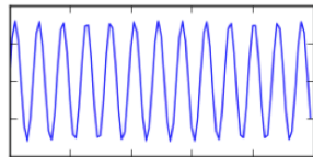
Time series
