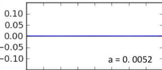
Time Asymmetry
