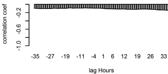
Cross-corr LP-ratio CPP
