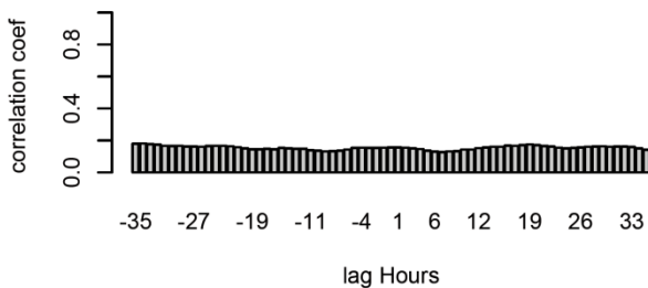
Cross-corr Glucose CPP
