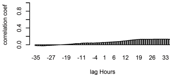
Cross-corr Glycerol CPP
