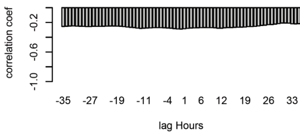
Cross-corr LG-ratio CPP
