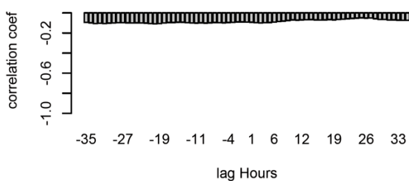
Cross-corr Lactate CPP
