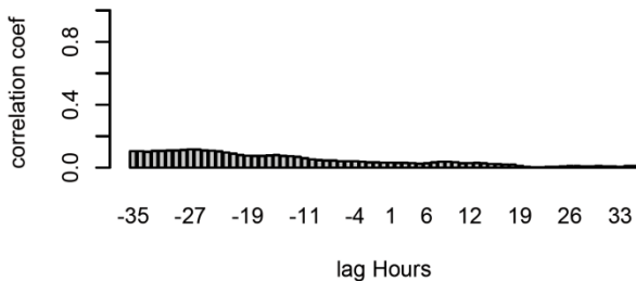
Cross-corr Pyruvate CPP
