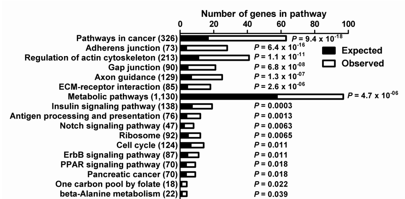
Supplementary Figure 1: Results from KEGG pathway analysis using genes that exhibit differential DNA methylation ( P < 0.05 ) after palmitate treatment in human pancreatic islets. Includes only pathways which also displayed enrichment for genes with differential expression after palmitate treatment in human pancreatic islets.
