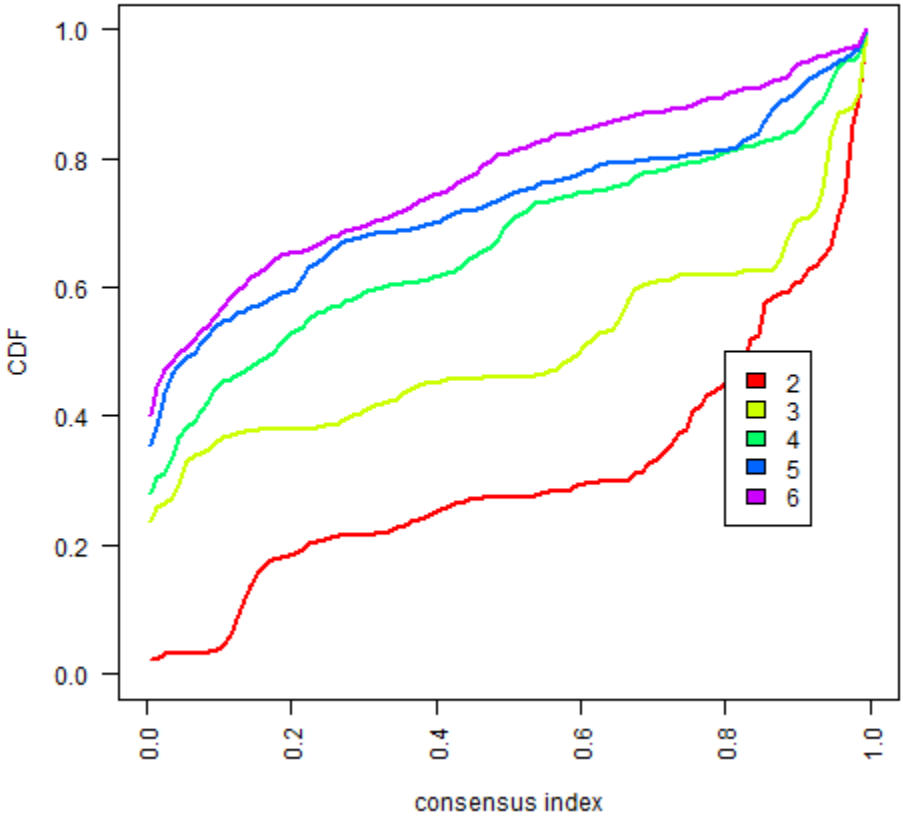
consensus CDF
