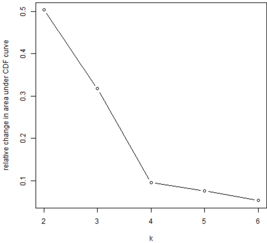
Delta area
