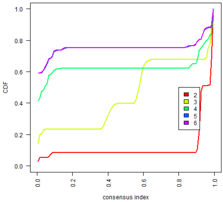
consensus CDF
