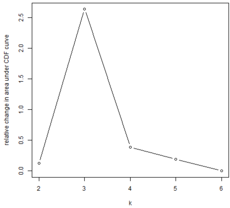
Delta area
