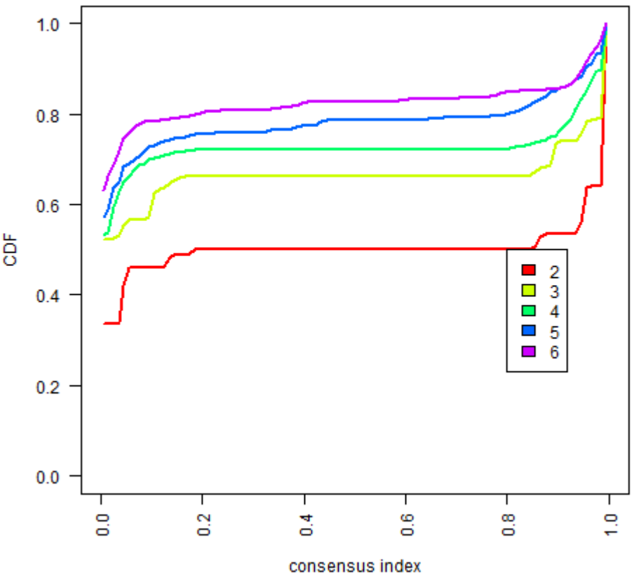
consensus CDF
