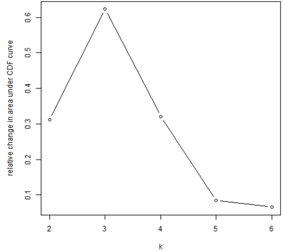
Delta area
