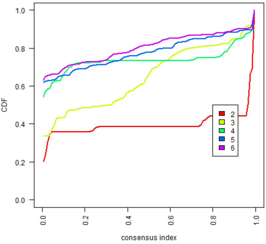
consensus CDF
