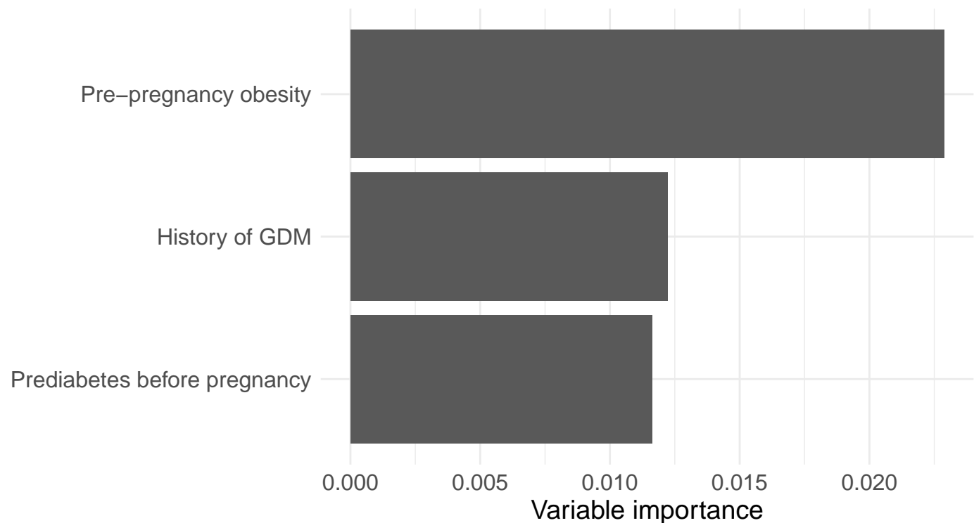
CART using predictors at levels 1–2
