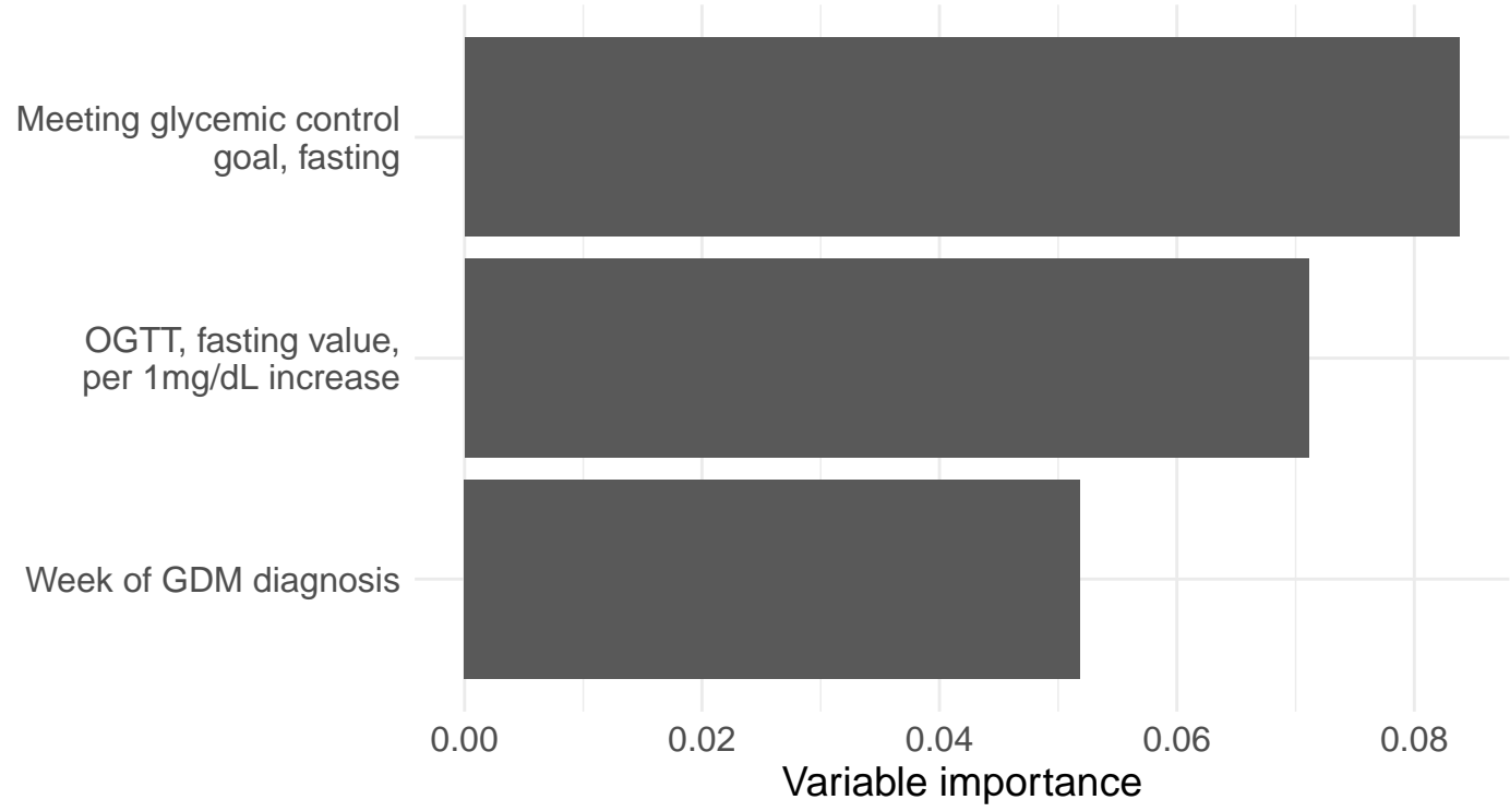
CART using predictors at levels 1–4
