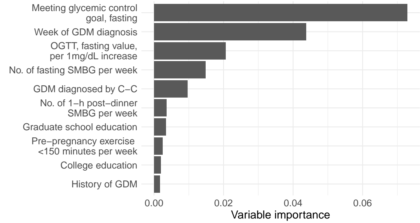
Simple super learner using predictors at levels 1–4
