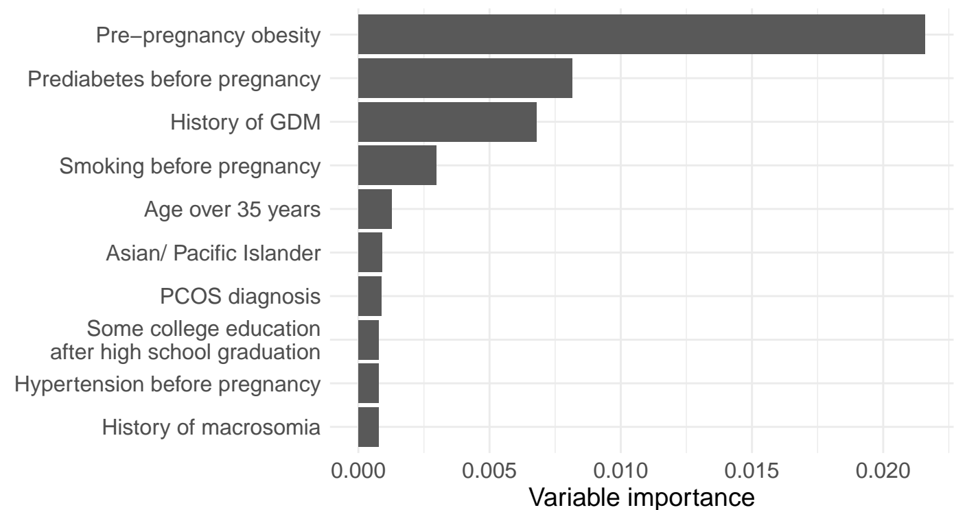
Simple super learner using predictors at levels 1–2
