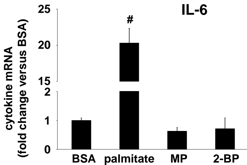
palmitic acid
