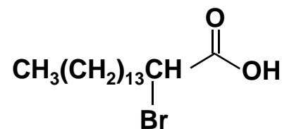
2-bromopalmitic acid
