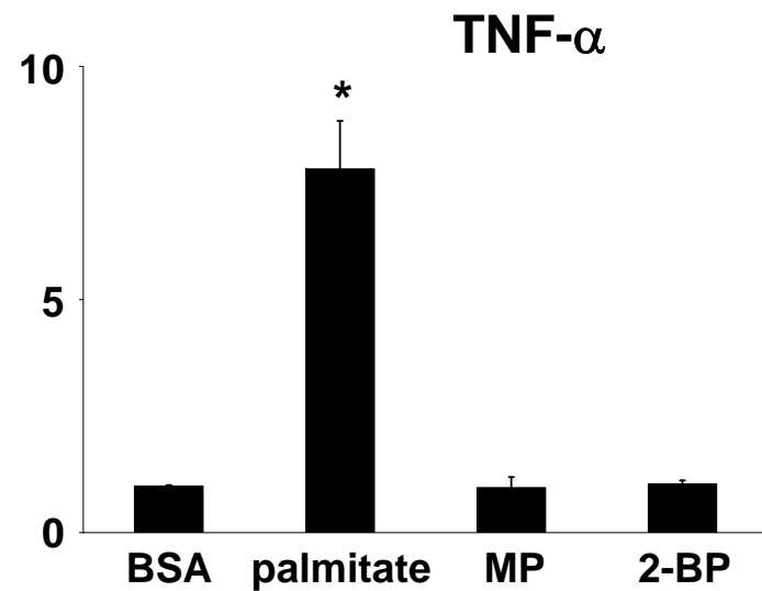
methyl palmitate
