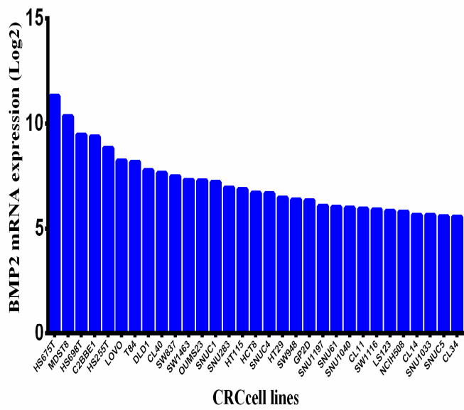
Supplementary figure 4. BMP2 expression in CRC cell lines from the Cancer Cell Line Encyclopedia. Data are presented as mRNA expression (Log2).
