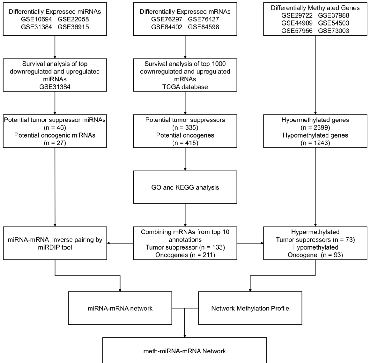
Fig. S1 Flowchart of constructing meth-miRNA-mRNA network.
