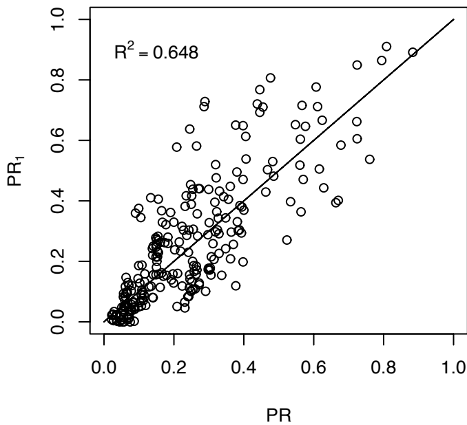
Interpolation, z = 1.5
