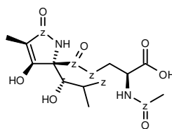
Lactacystin
