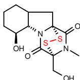
Gliotoxin
