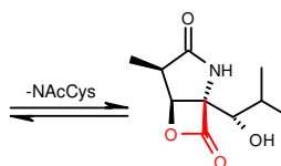
Clasto-lactacystin-β-lactone (omuralide)
