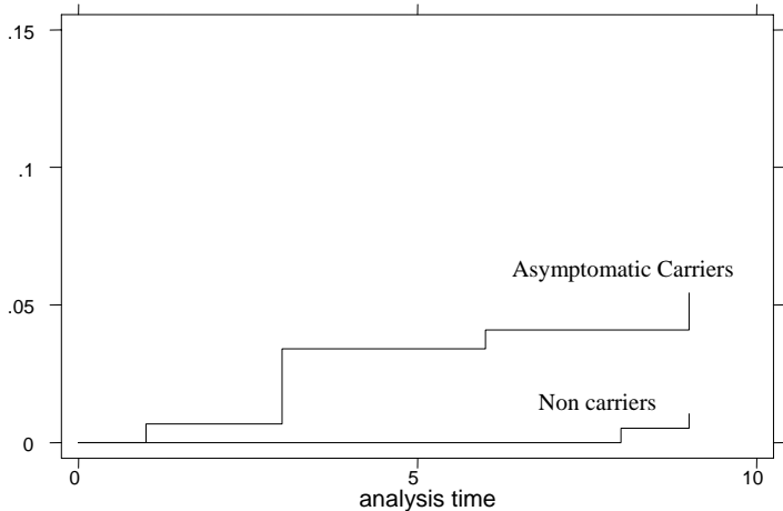
Kaplan-Meier survival estimates, by carriage
