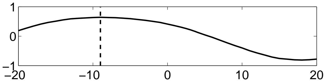
Minimum temperature
