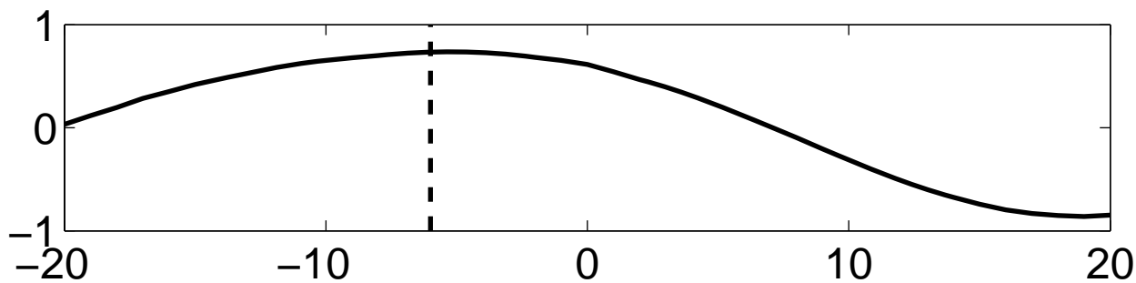
Maximum temperature
