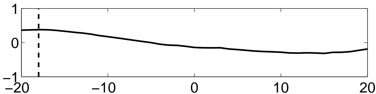
Precipitation
