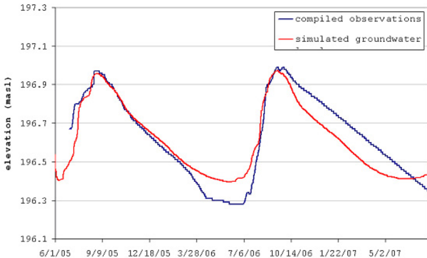
Zindarou GW level compared to estimate GW level from composite field observations
