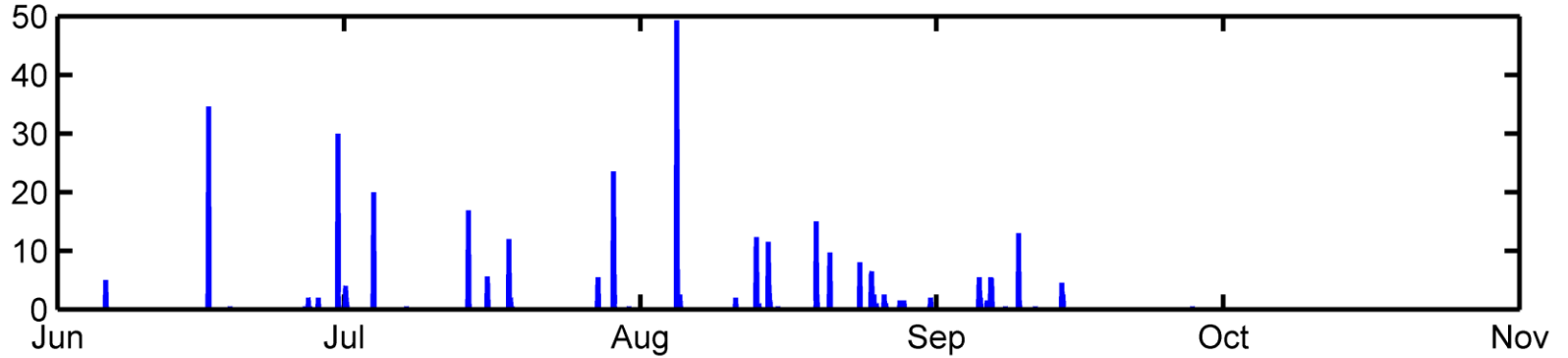
2007 Observed Hourly Rainfall
