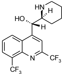
(-)-Mefloquine-enantiomer (-)-(11 S , 12 R )
