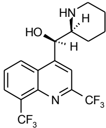
(+)-Mefloquine-enantiomer (+)-(11 R , 12 S )
