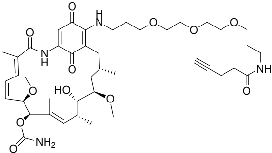
17-PEG-Alkyn-GA
