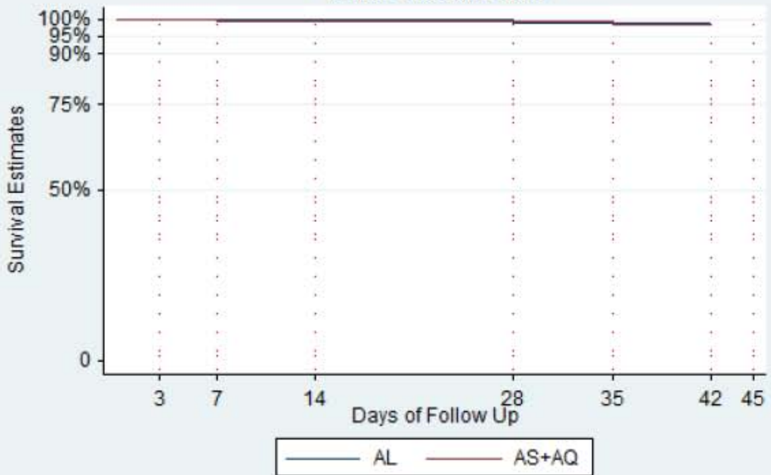
PCR-adjusted Kaplan-Meier Survival Curve without data correction
