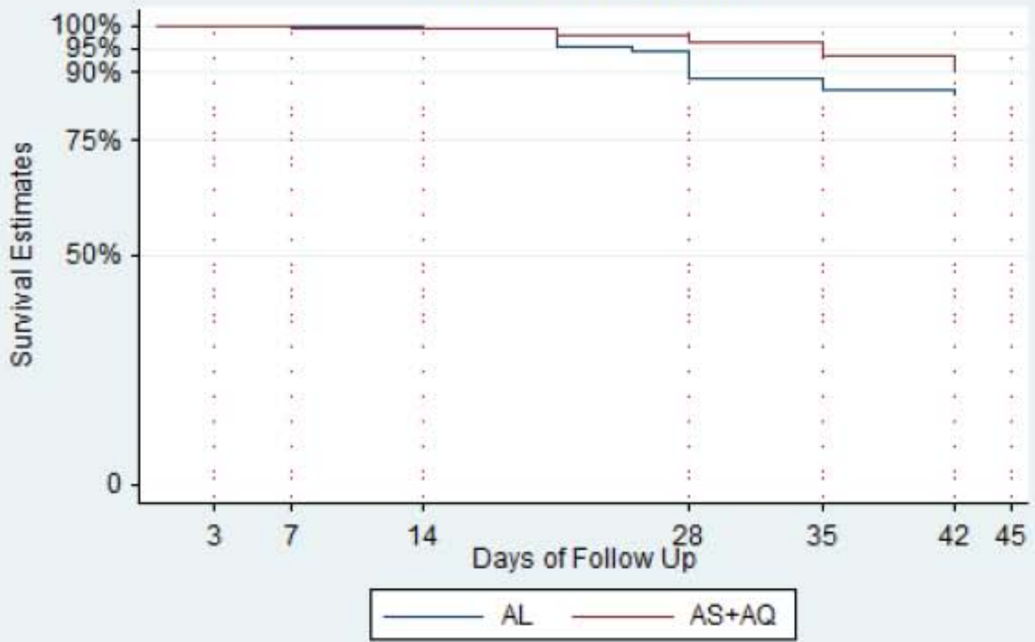
PCR-unadjusted Kaplan-Meier Survival Curve without data correction
