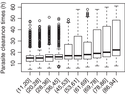
PQ EC 50 concentration (ng/mL) deciles
