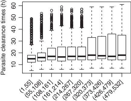
DHA EC 50 concentration (ng/mL) deciles
