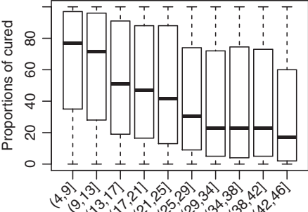
ART EC 50 concentration (ng/mL) deciles
