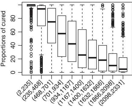
LF EC 50 concentration (ng/mL) deciles
