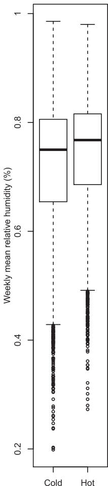
Relative humidity
