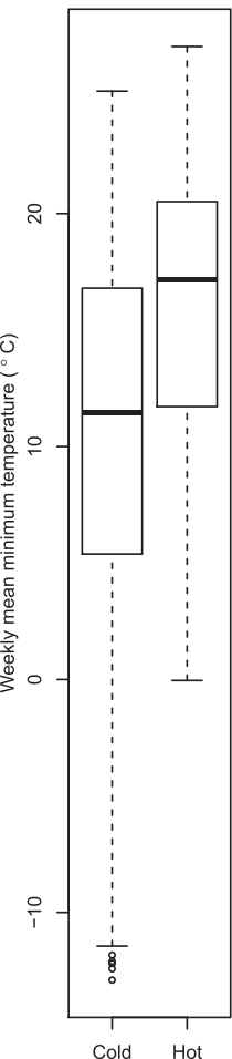
Minimum temperature
