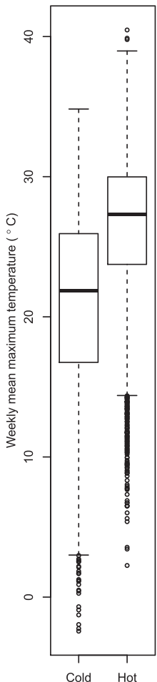
Maximum temperature
