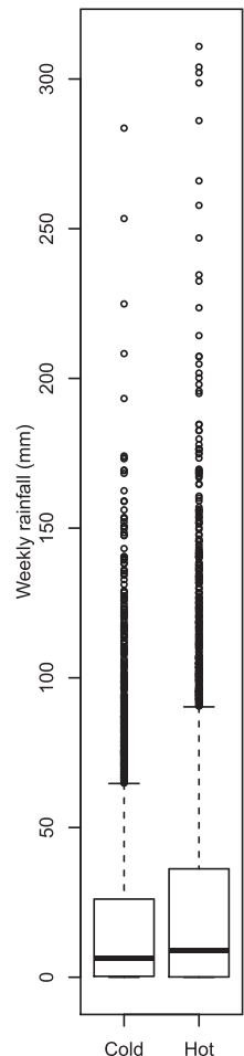
Rainfall
