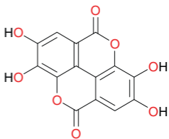
Ellagic acid (43)
