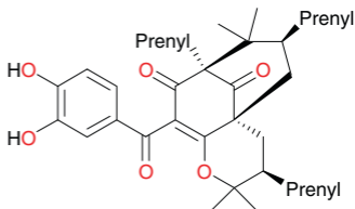
Isoxanthochymol (45)
