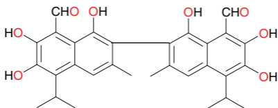
Gossypol (46)
