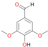
Syringaldehyde (44)
