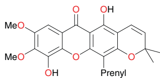
Gaboxanthone (84)
