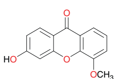
5-Hydroxy-3-methoxyxanthone (76)
