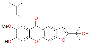
Pentadexanthone (87)
