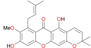
Garciniafuran (79)
