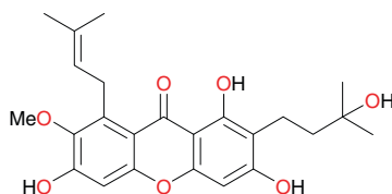
Cratoxylone (88)
