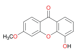
5-Hydroxy-3-methoxyxanthone (76)
