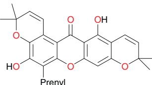
Tovophyllin A (80)
