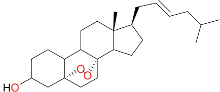
ergosterol-5,8-endoperoxide ( 91 )
