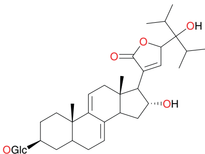
vernonioside B1 R_1 = \text{H} , R_2 = \text{OH} ( 95 )
