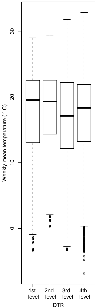
Mean temperature
