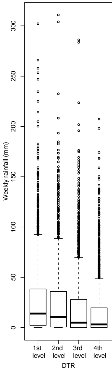
Rainfall
