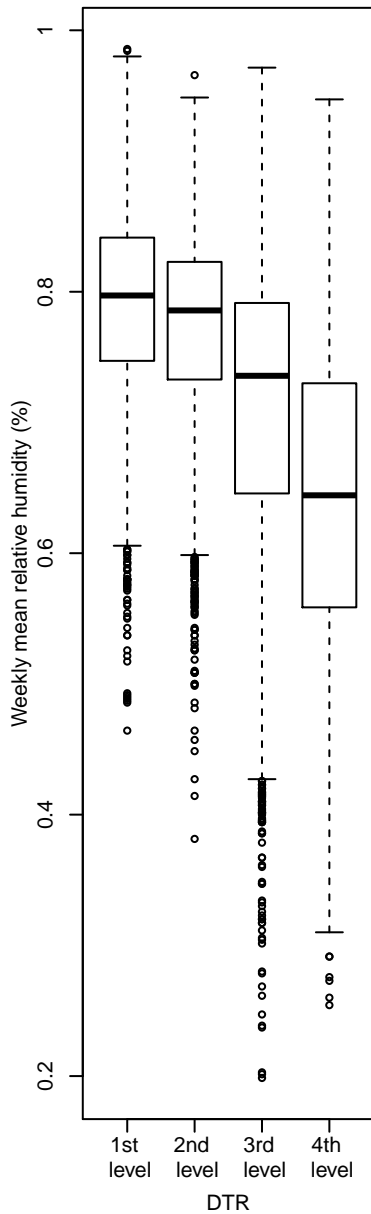
Relative humidity
