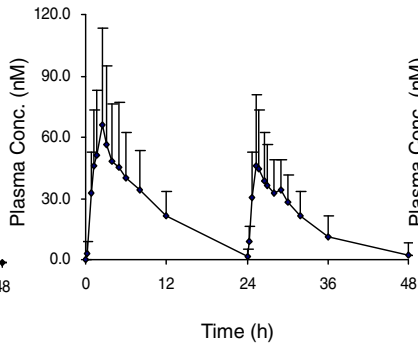
(Dihydroxylated QHS, M3)
