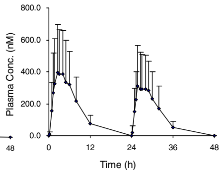
(Dihydroxylated QHS, M3)
