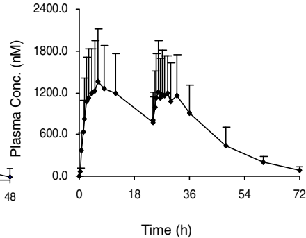
(Monohydroxylated deoxy-QHS, M1)
