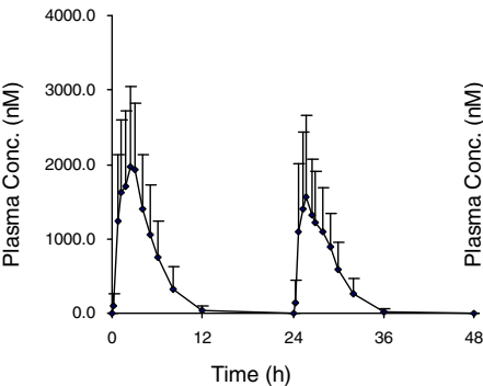
(Monohydroxylated QHS, M2)
