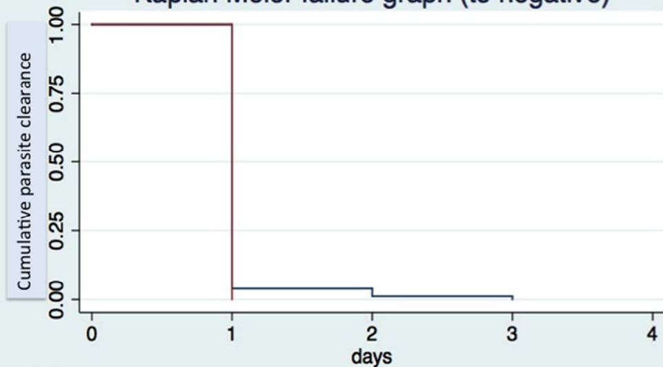
Kaplan Meier failure graph (to negative)
