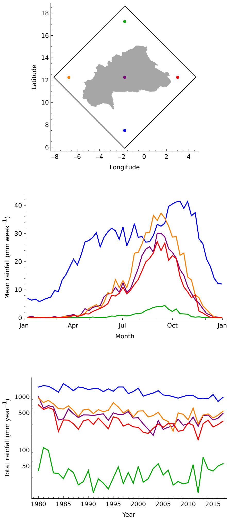
Figure S1: Rainfall across the simulation area. (b) and (c) plot rainfall profiles for five locations across the simulation region marked as points in (a)
