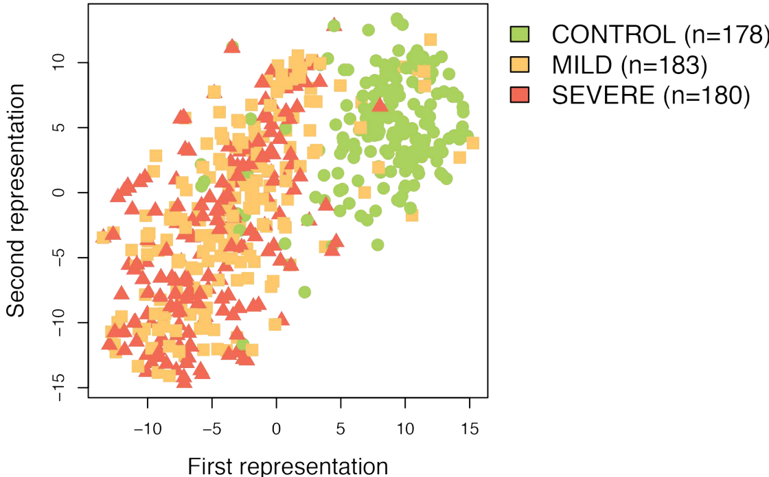
Sample subgroup
