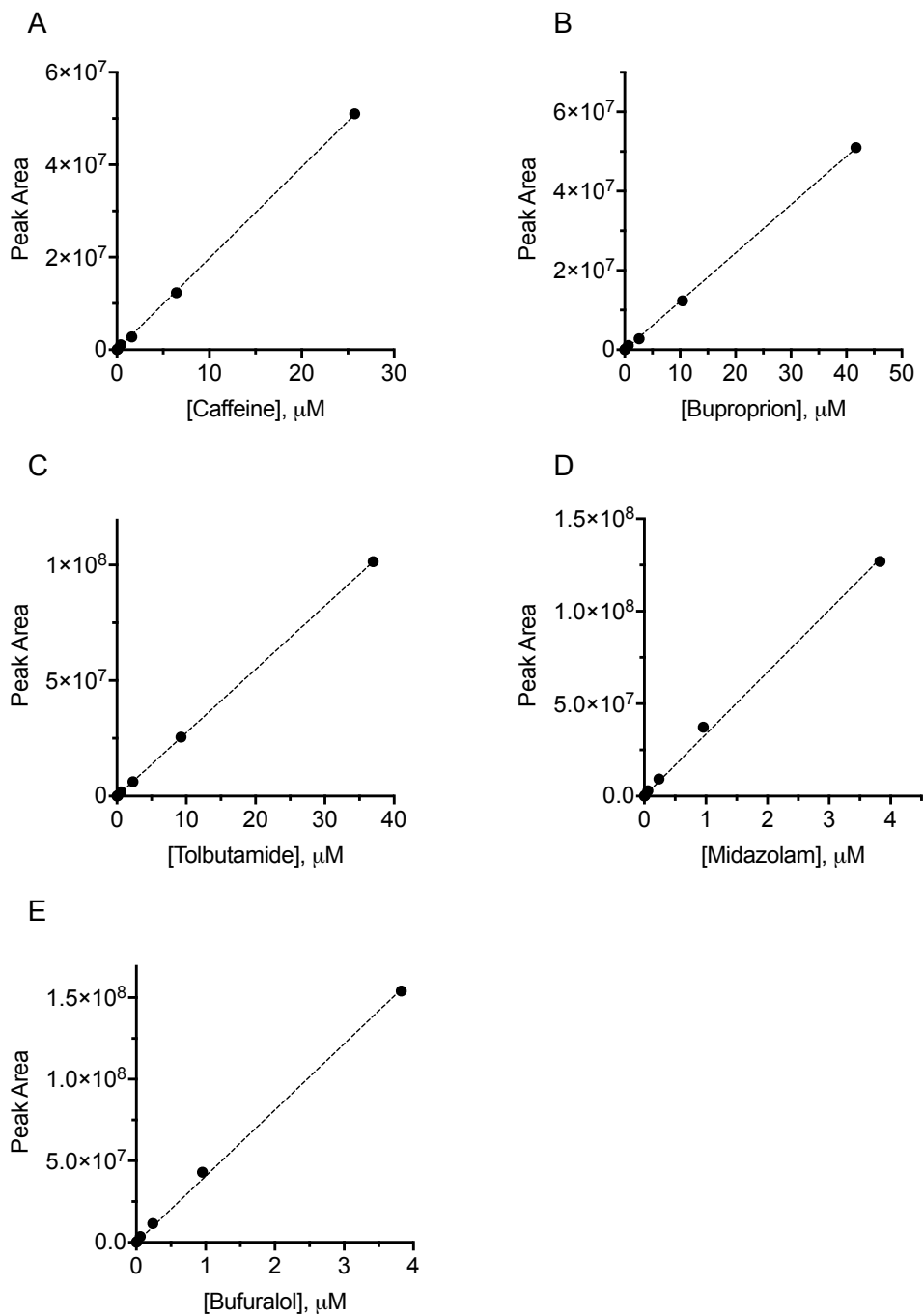
Figure S1. Standard curves for caffeine, bupropion, tolbutamide, midazolam and bufuralol measured by HILIC/MS. The drugs were spiked into naïve blood and processed identically to the experimental samples.
