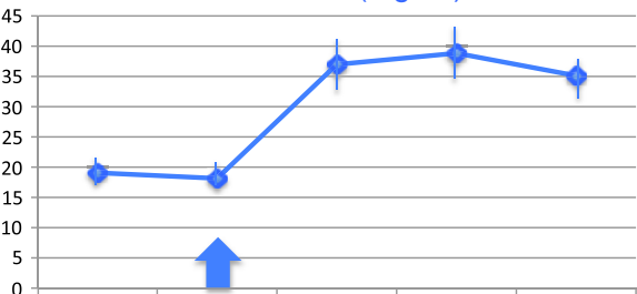
Leucine (mg/dL)
