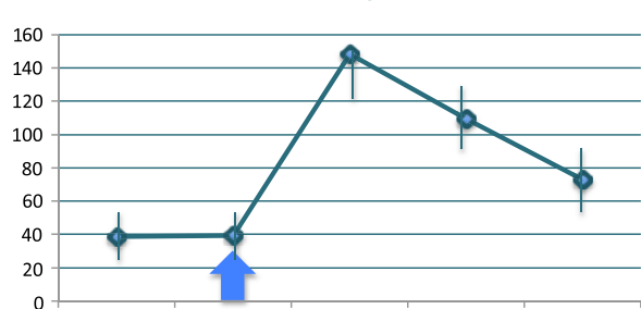
GIP (pg/mL)
