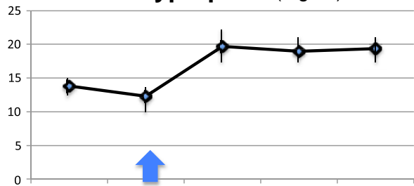
Tryptophan (mg/dL)
