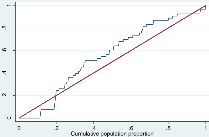
— Conc curve (child mortality <9 months) — Equality line
